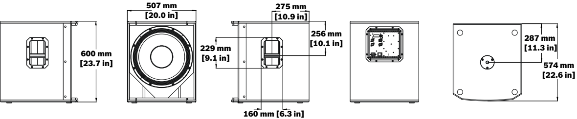
Figure 9.5: ELX200-18SP dimensions
