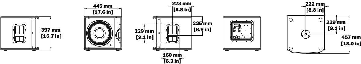
Figure 9.4: ELX200-12SP dimensions
