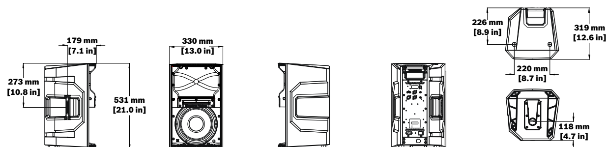
Figure 9.1: ELX200-10P dimensions
