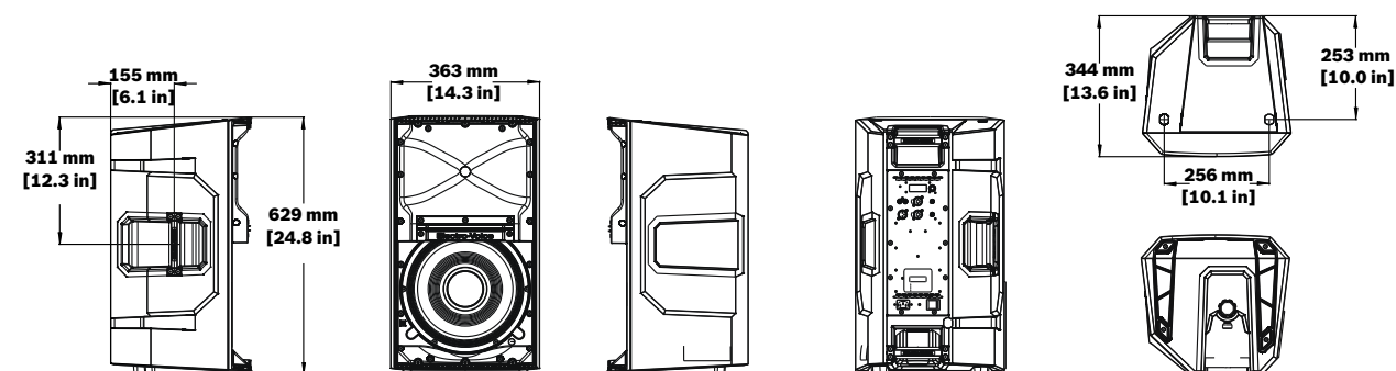
Figure 9.2: ELX200-12P dimensions
